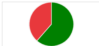
Short Profit/Loss
