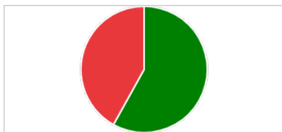
Long Profit/Loss
